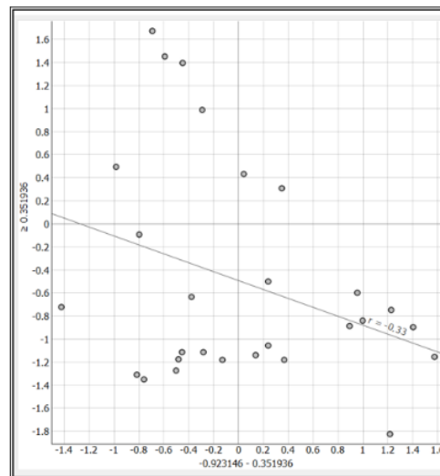
Figure 3 Discretization-three interval-lasso
