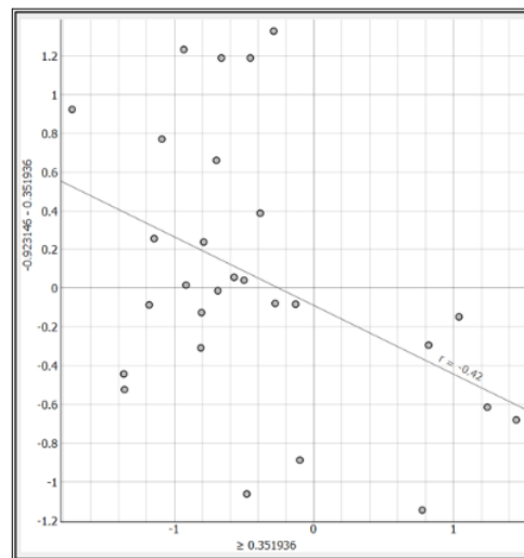
Figure 4 Discretization-three interval-ridge
